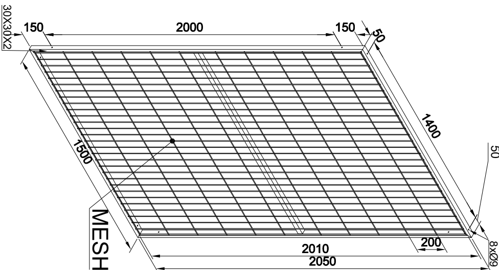
ISOMETRIC VIEW
