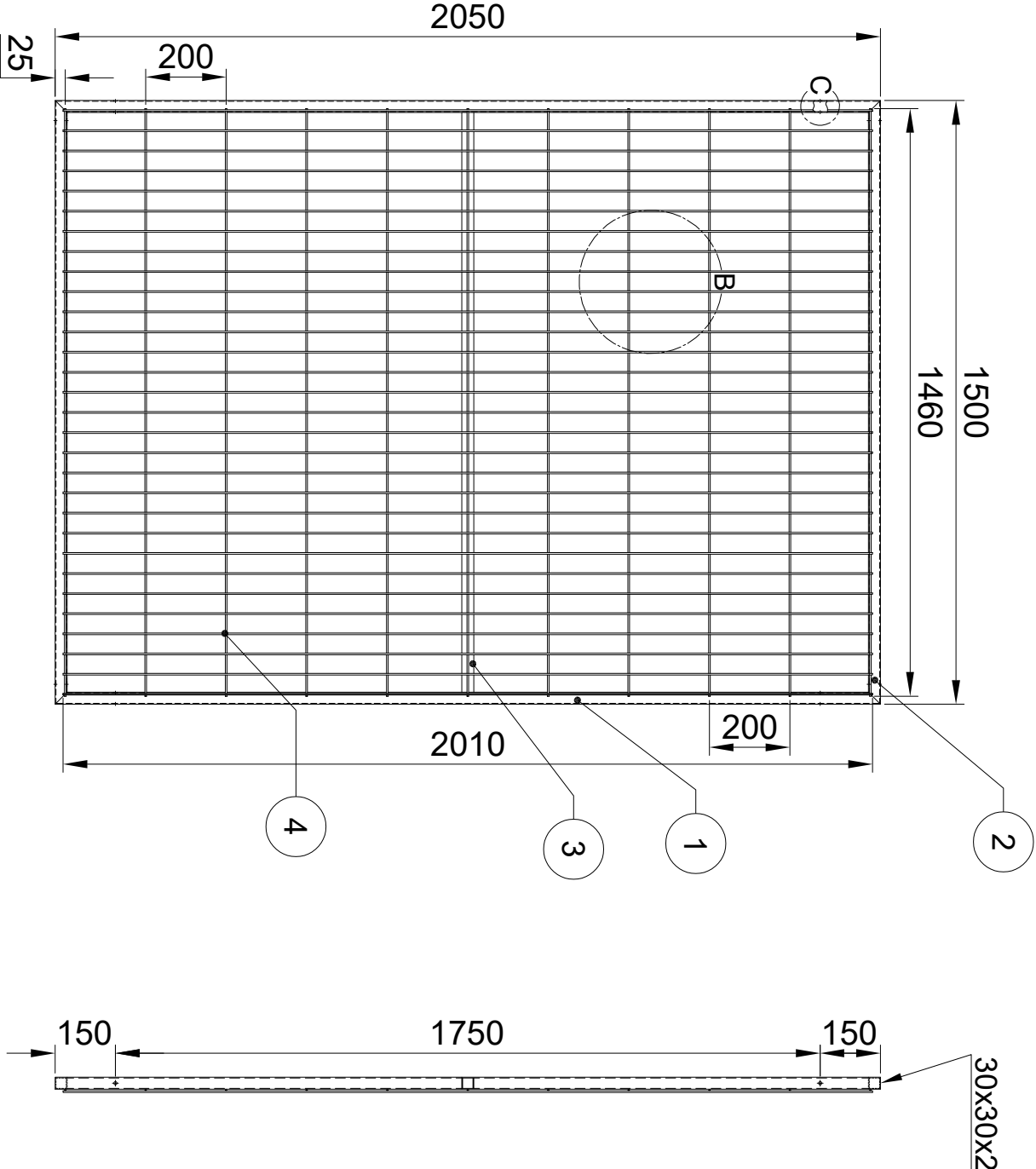
ELEVATION VIEW
