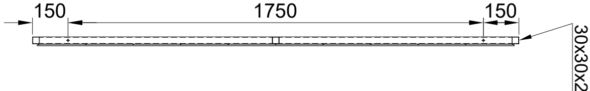
SIDE VIEW
