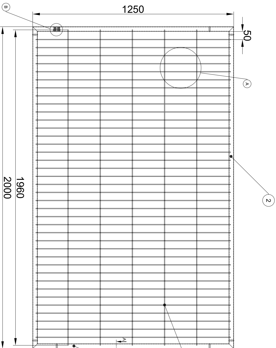
ELEVATION VIEW
