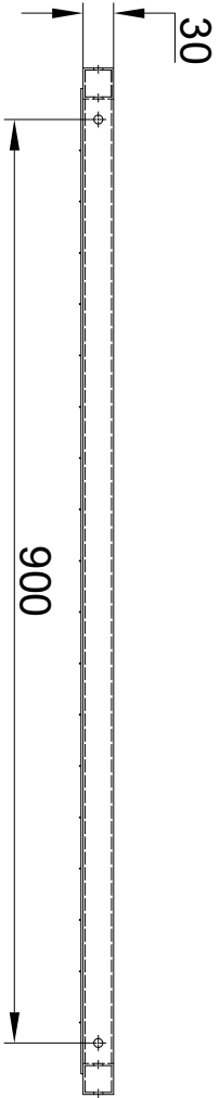
ELEVATION VIEW
