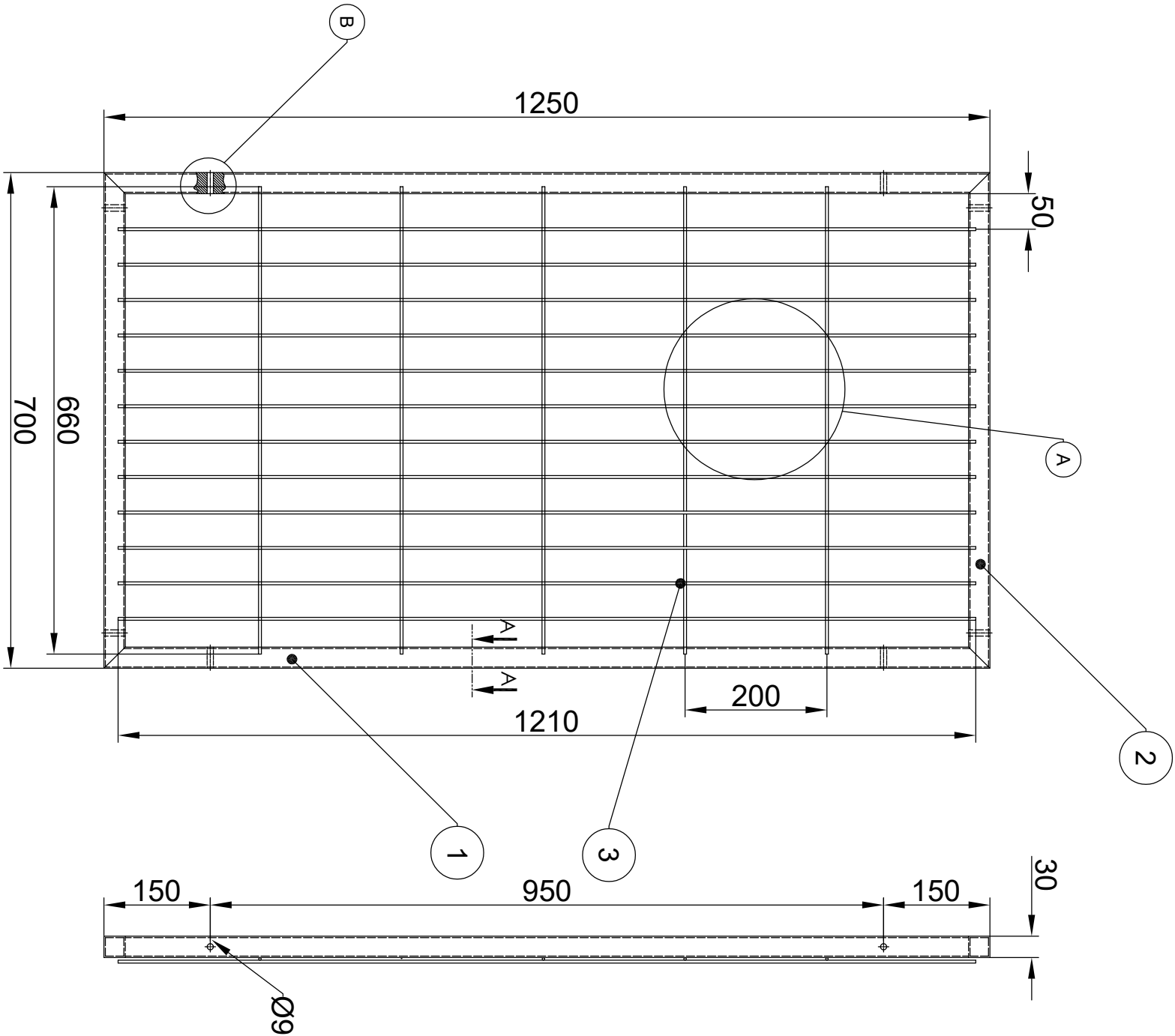
ELEVATION VIEW
