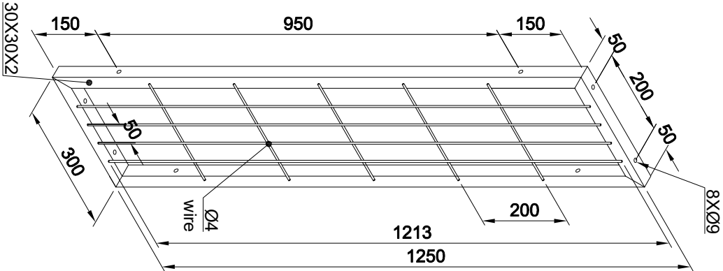
ISOMETRIC
